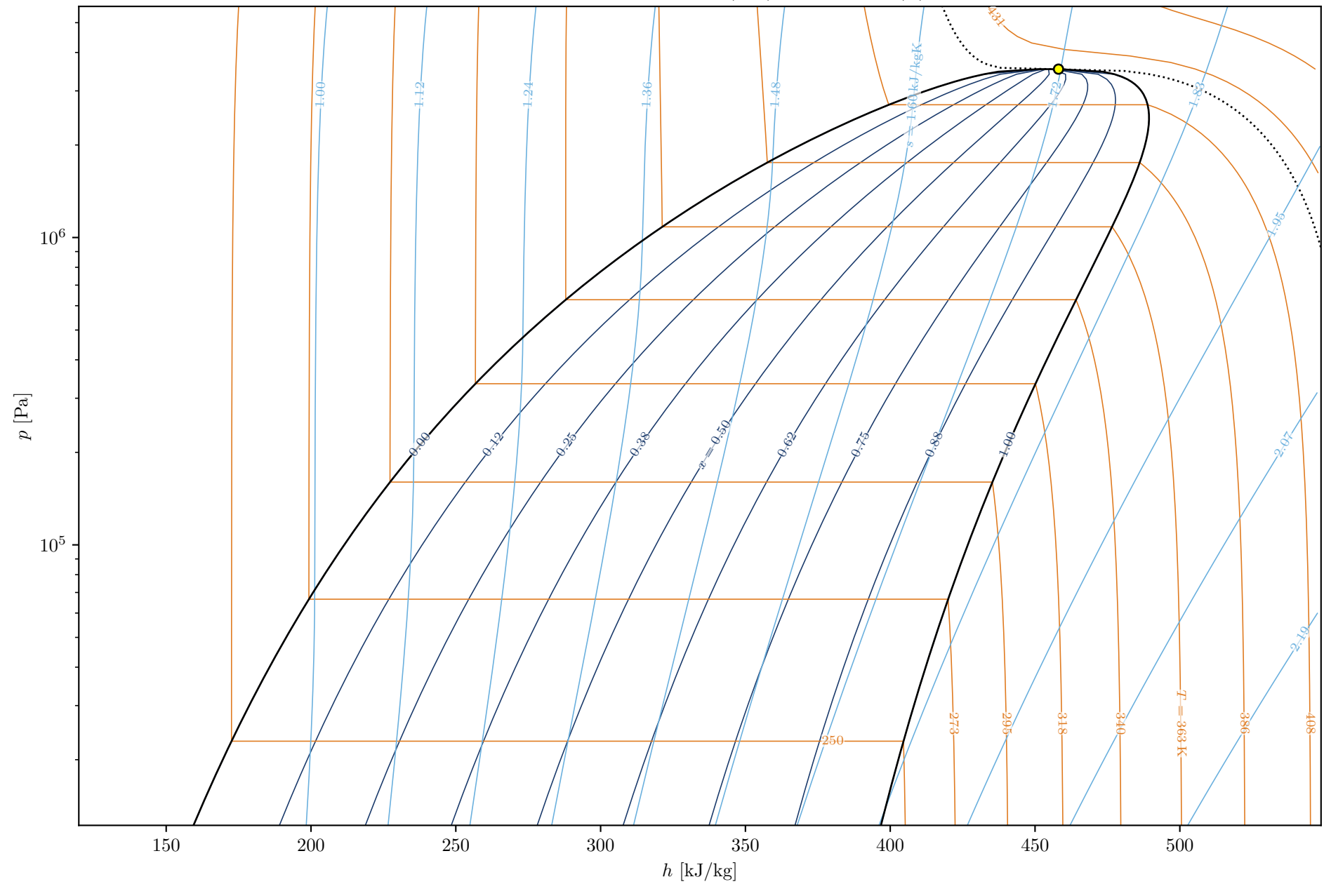
Thermodynamic Diagram (PH) – R1234ze(Z)
